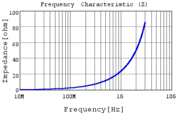
LQG15HN3N9B02 |Z|
