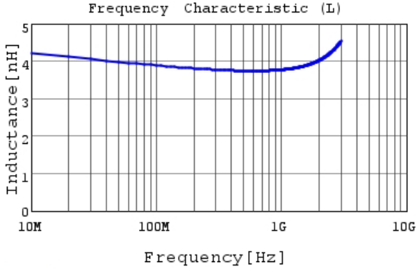
LQG15HN3N9B02 L
