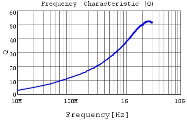
LQG15HN3N9B02 Q
