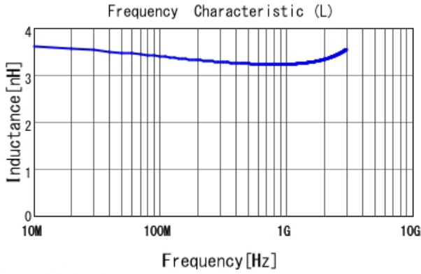
LQP03TN3N2BZ2 L
