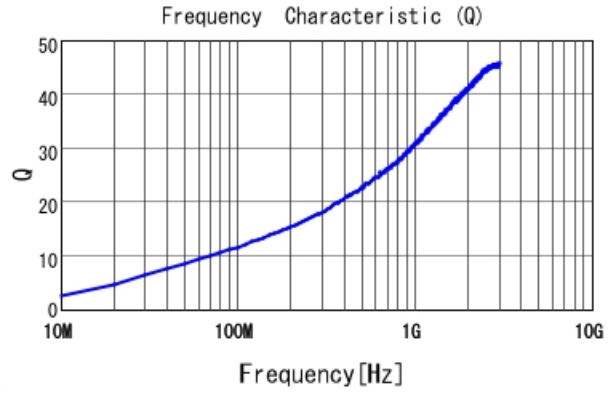
LQP03TN3N2BZ2 Q
