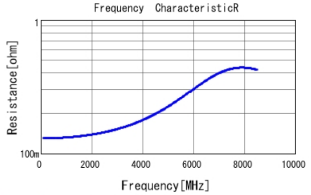
GJM0335C1E3R3WB01 R DCOV, 25degC
