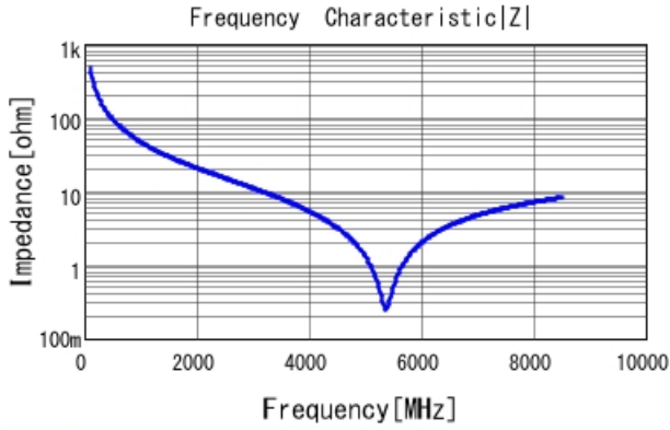
GJM0335C1E3R3WB01 |Z| DCOV, 25degC
