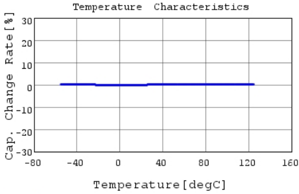
GQM1875C2E3R6BB12 C-Temp. capchange, DCOV, 1
