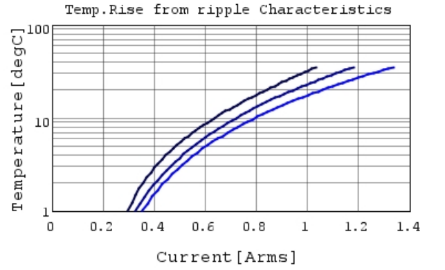
GQM1875C2E3R6BB12 Temp.rise — 1GHz — 2
