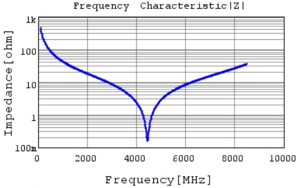
GQM1875C2E3R6BB12 |Z| DC0V, 25degC
