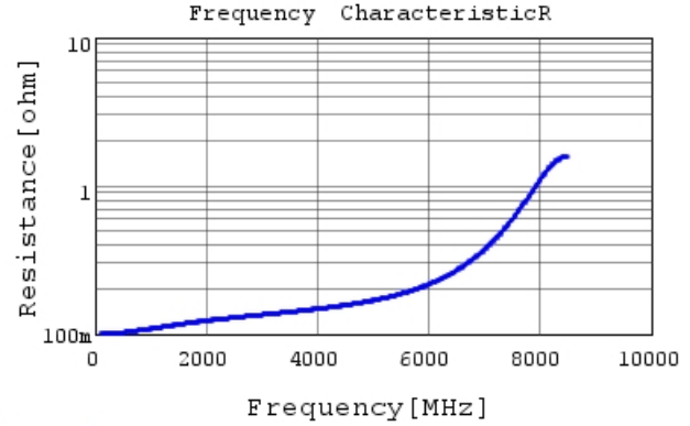
GQM1875C2E3R6BB12 R DC0V, 25degC
