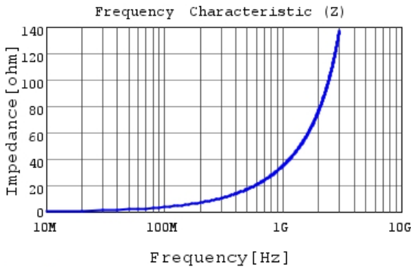
LQG18HN5N6S00 |Z|
