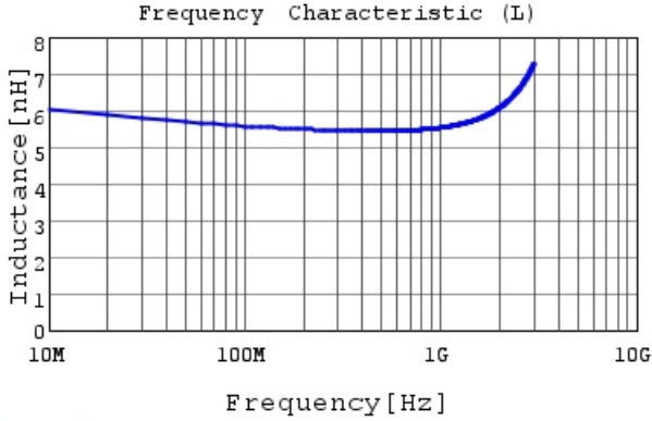
LQG18HN5N6S00 L
