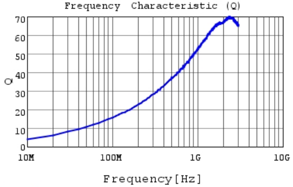
LQG18HN5N6S00 Q
