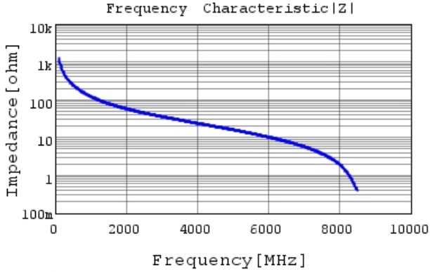
GJM0335C1E1R3CB01 |Z| DCOV, 25degC
