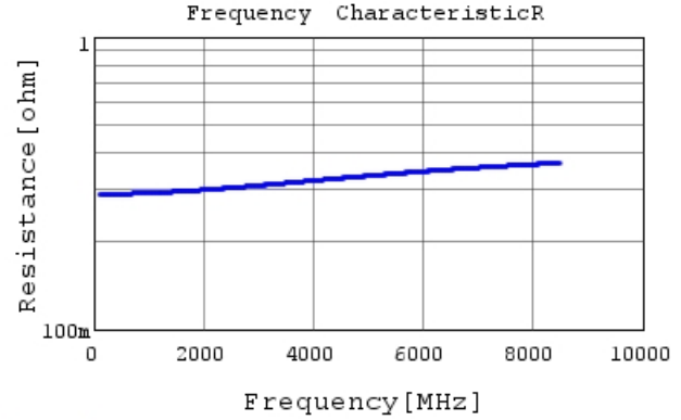
GJM0335C1E1R3CB01 R DCOV, 25degC
