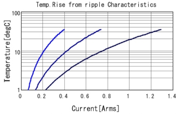
GR331BD72W333KW01 Temp. rise — 30kHz — 100kHz
