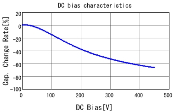
GR331BD72W333KW01 C-DC bias capchange, 25.0degC, A
