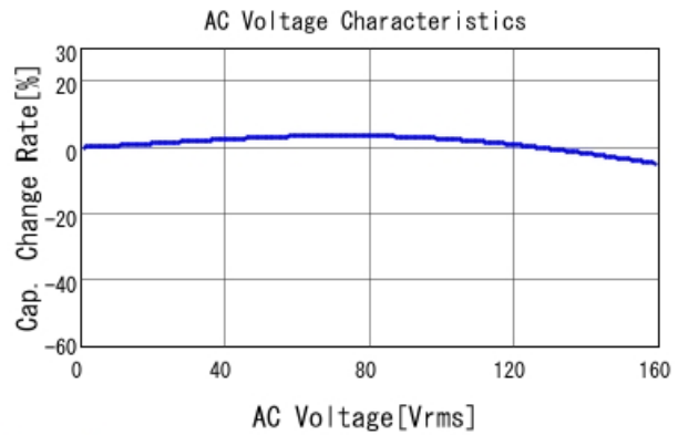
GR331BD72W333KW01 C-AC Voltage capchange, DCOV, 25
