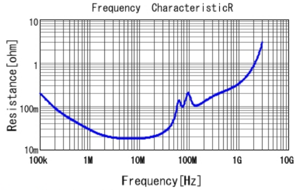
GR331BD72W333KW01 R DCOV, 25degC
