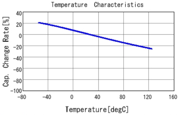
GR331BD72W333KW01 C-Temp. capchange, DCOV, AC1Vrms
