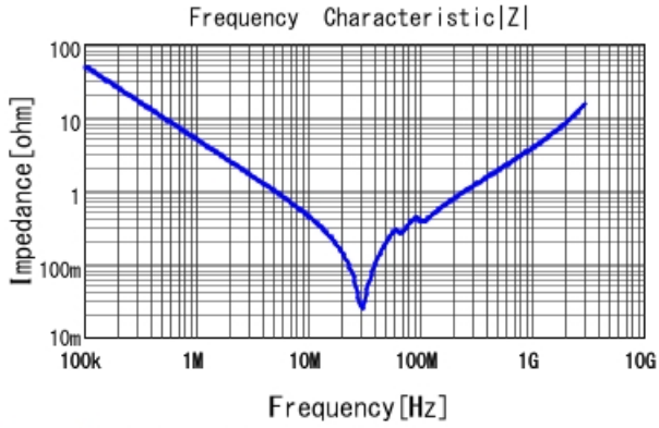
GR331BD72W333KW01 |Z| DCOV, 25degC
