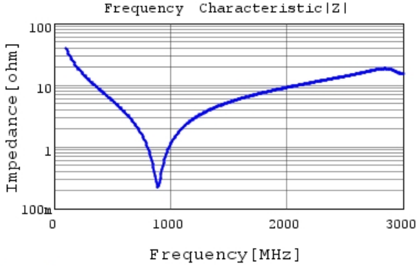
GRM31A5C2J390JW01 |Z| DC0V, 25degC
