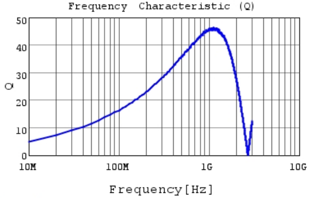
LQG18HN18NJ00 Q
