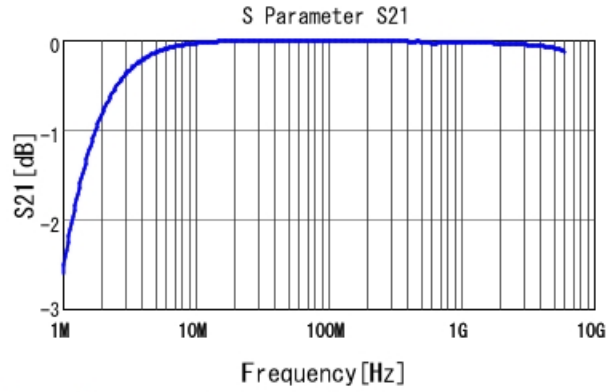
GRM1557U1A182JA01 S21 DCOV, 25degC
