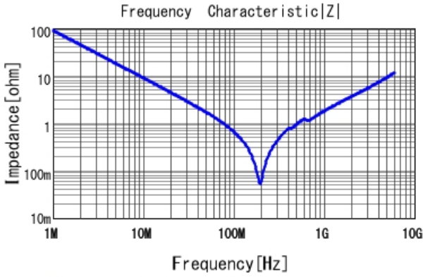
GRM1557U1A182JA01 |Z| DCOV, 25degC
