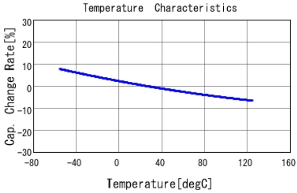
GRM1557U1A182JA01 C-Temp. capchange, DCOV, AC1Vrms
