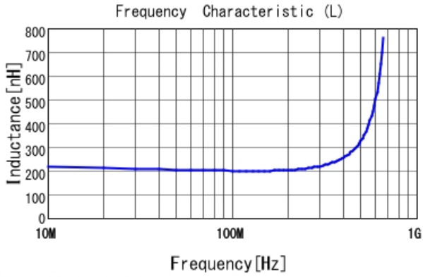
LQP03TNR20J02 L
