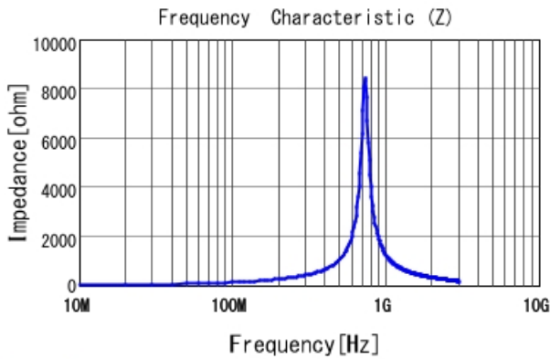
LQP03TNR20J02 |Z|
