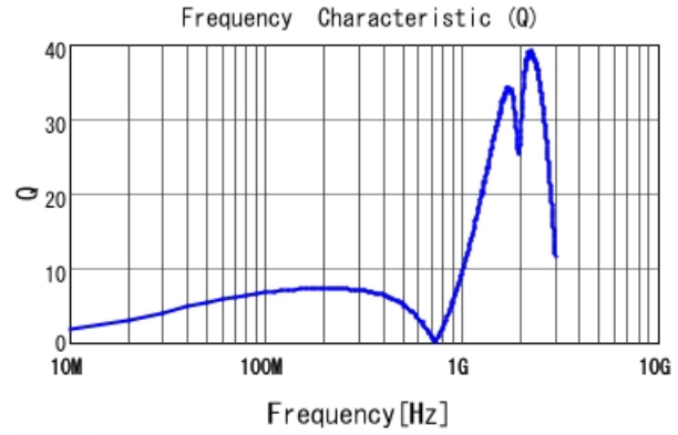
LQP03TNR20J02 Q
