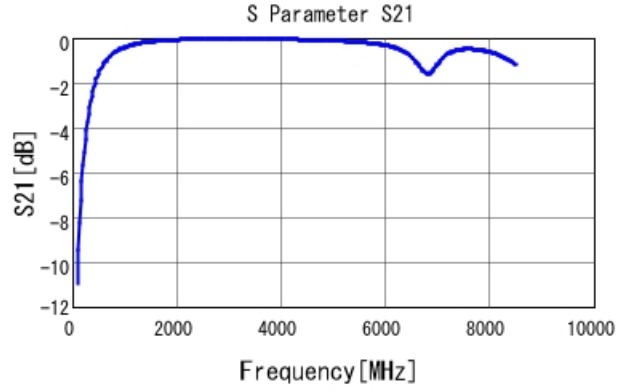
GCM1885C2A4R7BA16 S21 DC0V, 25degC
