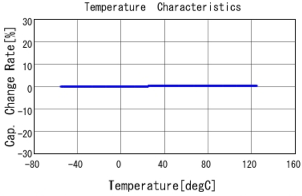
GCM1885C2A4R7BA16 C-Temp. capchange, DC0V, AC1Vrms
