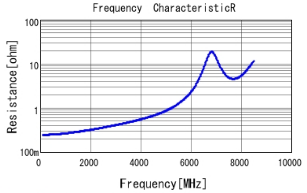
GCM1885C2A4R7BA16 R DCOV, 25degC
