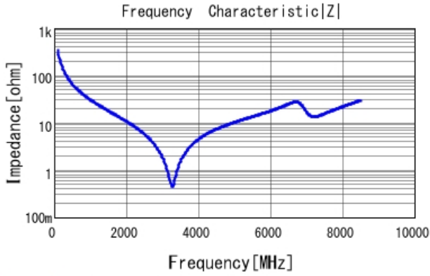
GCM1885C2A4R7BA16 |Z| DCOV, 25degC
