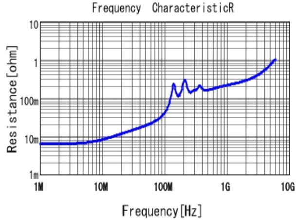
■ GRM1885C1H103JA01 R DCOV, 25degC
