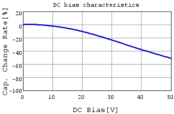
RDER71H104K0P1H03B C-DC bias capchange, 25.0
