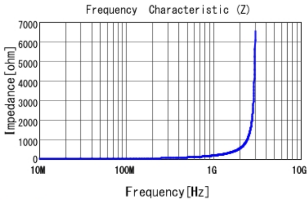
LQP03TN27NH02 |Z|
