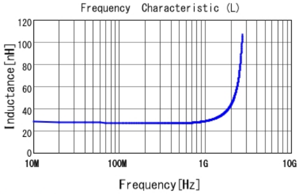
LQP03TN27NH02 L
