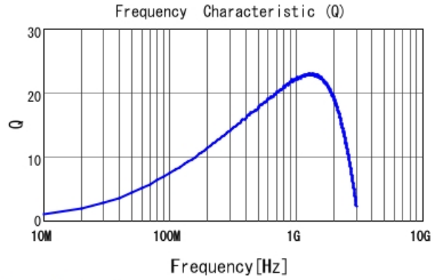
LQP03TN27NH02 Q
