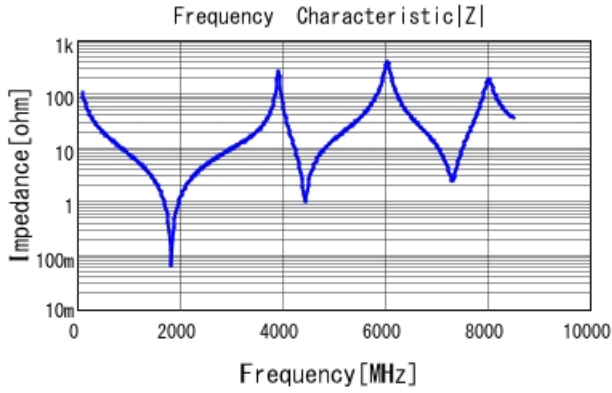
GQM22M5C2H150JB01 |Z| DCOV, 25degC
