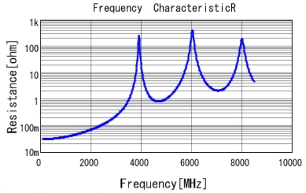
GQM22M5C2H150JB01 R DCOV, 25degC
