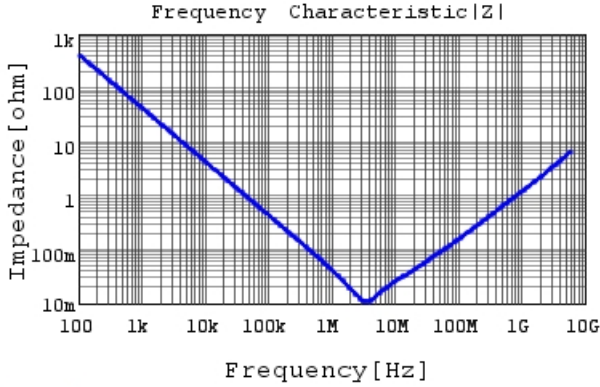
GRM155R61A475MEAA |Z| DCOV, 25degC
