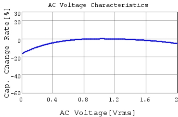
GRM155R61A475MEAA C-AC Voltage capchange, Dc
