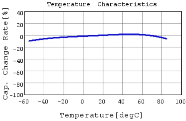
GRM155R61A475MEAA C-Temp. capchange, DC0.0V,
