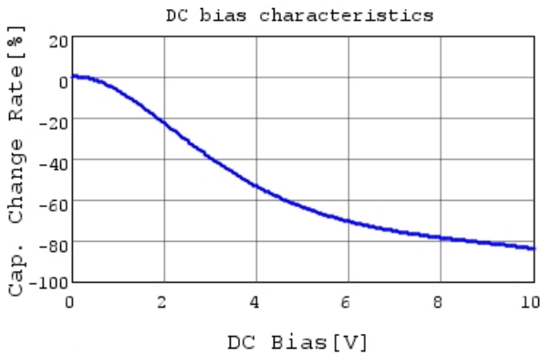
GRM155R61A475MEAA C-DC bias capchange, 25.0c
