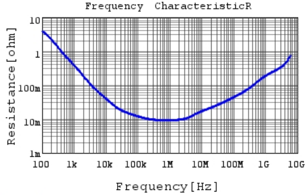
GRM155R61A475MEAA R DCOV, 25degC
