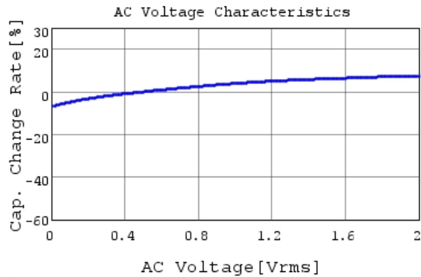
GRM033R61A123KE84 C-AC Voltage capchange, Dc
