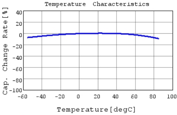
GRM033R61A123KE84 C-Temp. capchange, DC0.0V,
