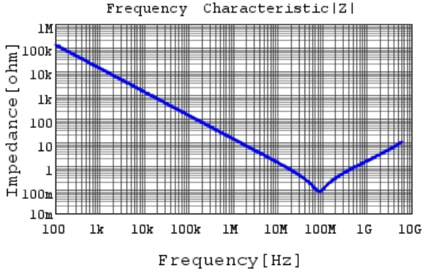
GRM033R61A123KE84 |Z| DCOV, 25degC
