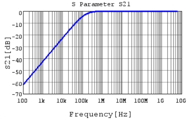
GRM033R61A123KE84 S21 DC0V, 25degC
