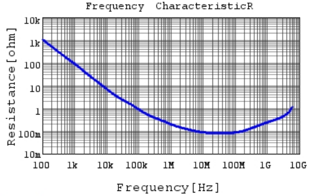
GRM033R61A123KE84 R DCOV, 25degC
