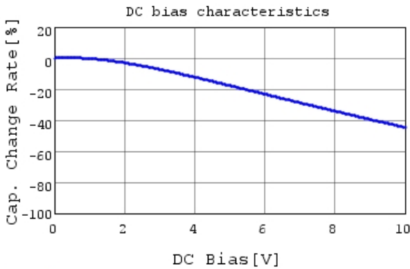
GRM033R61A123KE84 C-DC bias capchange, 25.0c
