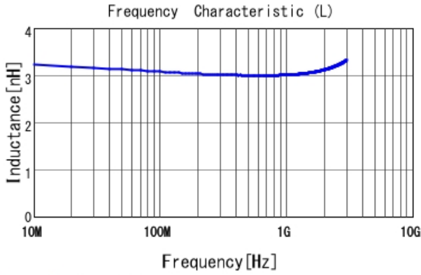
LQP03HQ3N0B02 L
