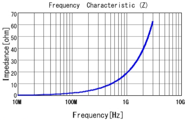
LQP03HQ3N0B02 |Z|
