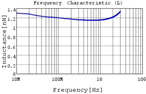
LQG15HS1N2B02 L
