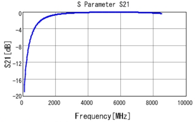
GRM1555C1H1R8BA01 S21 DCOV, 25degC
