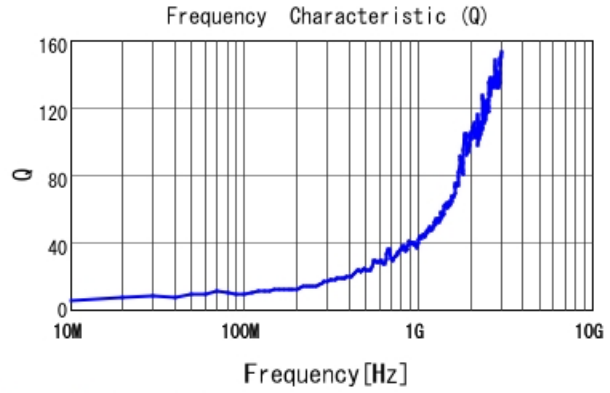
LQP03TG0N1B02 Q
