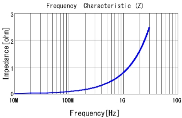
LQP03TG0N1B02 |Z|
