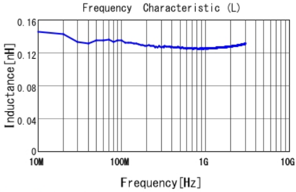
LQP03TG0N1B02 L
