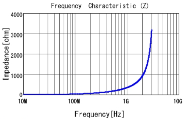
LQW15AN51NG0Z |Z|
