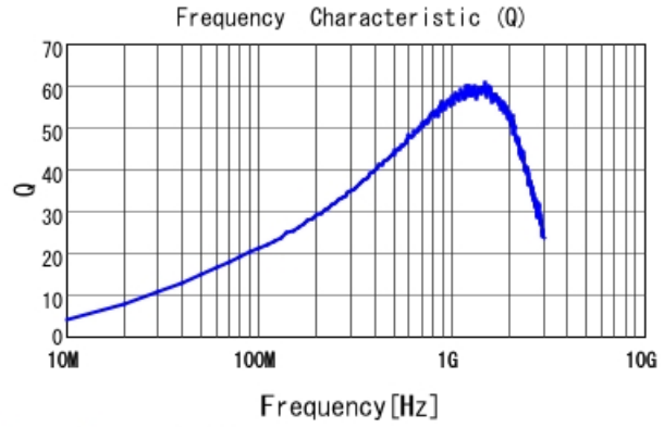
LQW15AN51NG0Z Q
