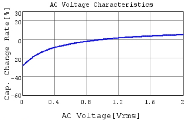
GRM188R61C475ME11 C-AC Voltage capchange, Dc
