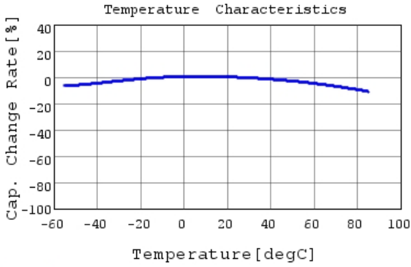
GRM188R61C475ME11 C-Temp. capchange, DC0.0V,
