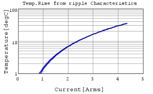
GRM188R61C475ME11 Temp.rise 500kHz
