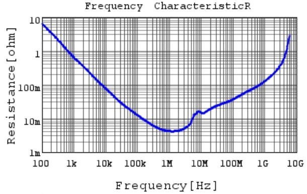
GRM188R61C475ME11 R DCOV,25degC
