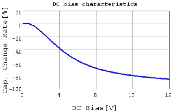
GRM188R61C475ME11 C-DC bias capchange, 25.0c
