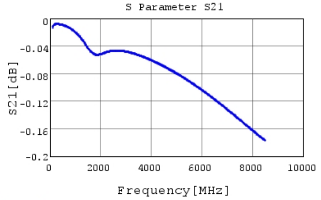
GRM0335C1E391JA01 S21 DCOV, 25degC
