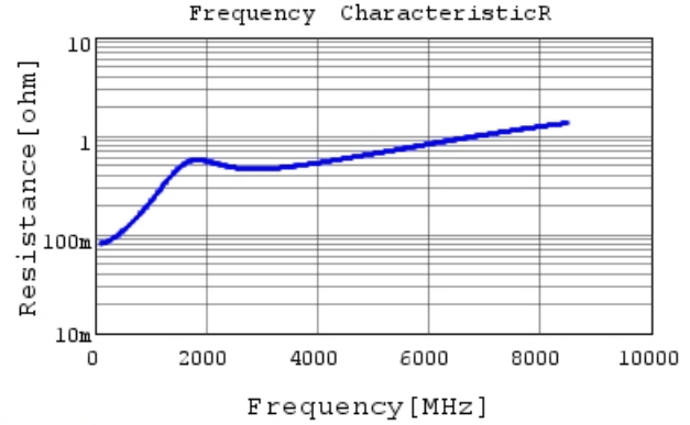
GRM0335C1E391JA01 R DCOV, 25degC
