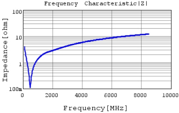
GRM0335C1E391JA01 |Z| DCOV, 25degC
