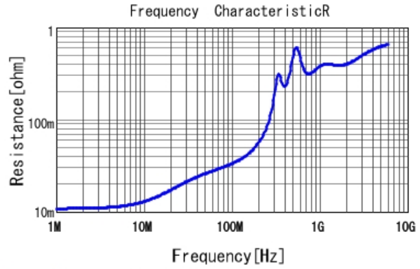
GRM2165C2A222JA01 R DCOV, 25degC
