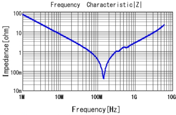
GRM2165C2A222JA01 |Z| DCOV, 25degC
