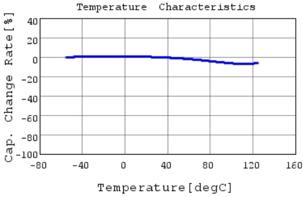
GRM033R71E471KA01 C-Temp. capchange, DC0.0V,
