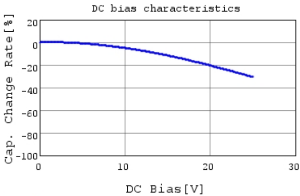
GRM033R71E471KA01 C-DC bias capchange, 25.0c
