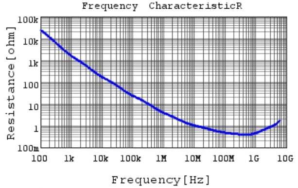
GRM033R71E471KA01 R DCOV, 25degC
