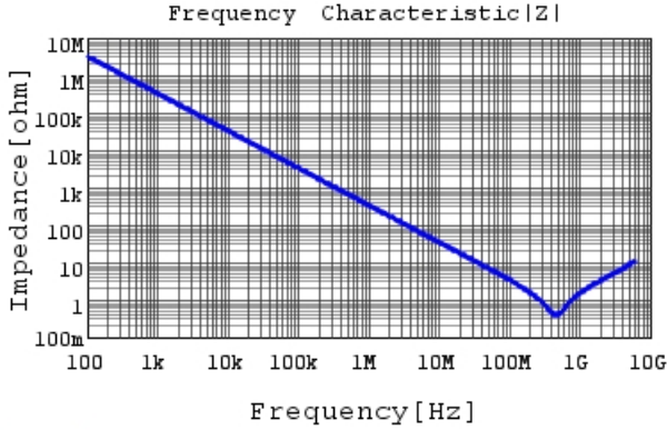
GRM033R71E471KA01 |Z| DCOV, 25degC
