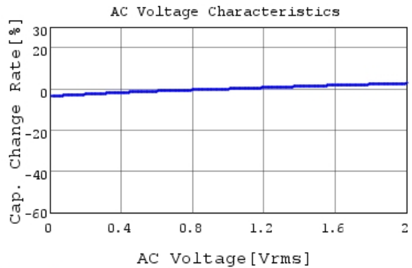
GRM033R71E471KA01 C-AC Voltage capchange, Dc
