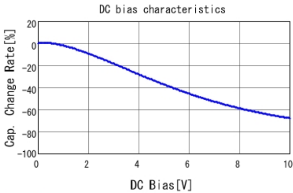
GRM155R61A105KE15 C-DC bias capchange, 25.0degC, A
