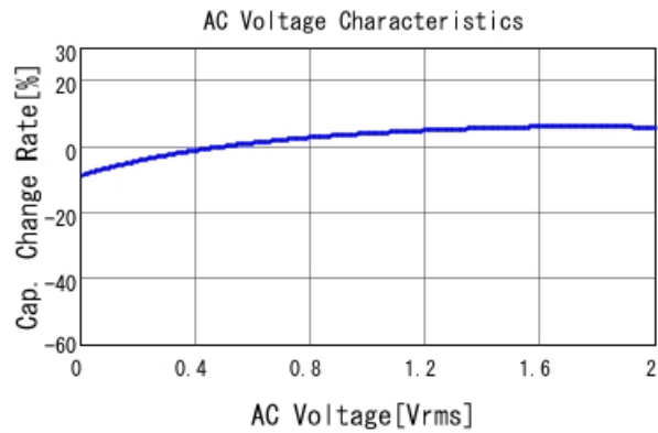
GRM155R61A105KE15 C-AC Voltage capchange, DCOV, 25
