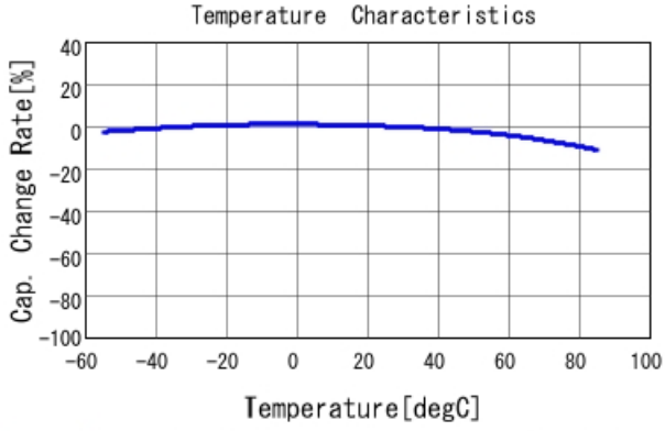
GRM155R61A105KE15 C-Temp. capchange, DC0.0V, AC0.5
