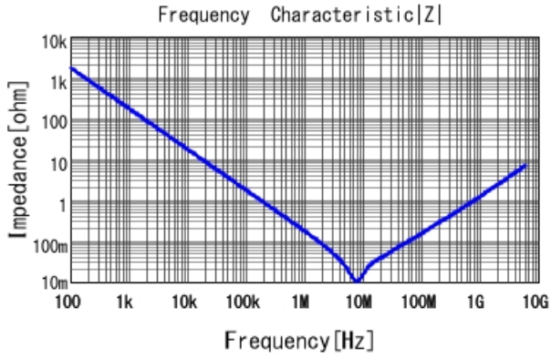
GRM155R61A105KE15 |Z| DCOV, 25degC
