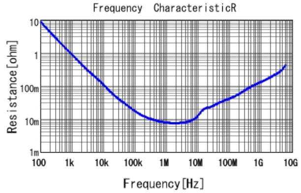
GRM155R61A105KE15 R DCOV, 25degC
