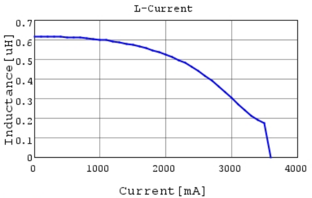
LQH2HPZR68MGR L-Current 20degC
