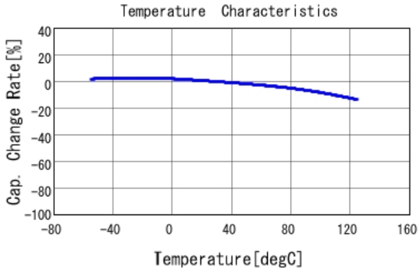
GRM21BR71H105KA12 C-Temp. capchange, DC0.0V, AC1.C
