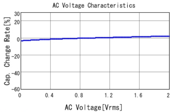
GRM155R71H392KA01 C-AC Voltage capchange, DCOV, 25
