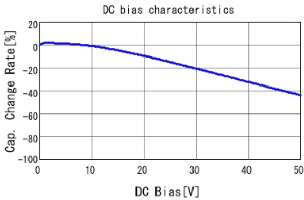
GRM155R71H392KA01 C-DC bias capchange, 25.0degC, A
