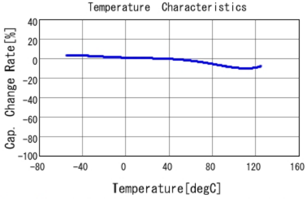
GRM155R71H392KA01 C-Temp. capchange, DC0.0V, AC1.C
