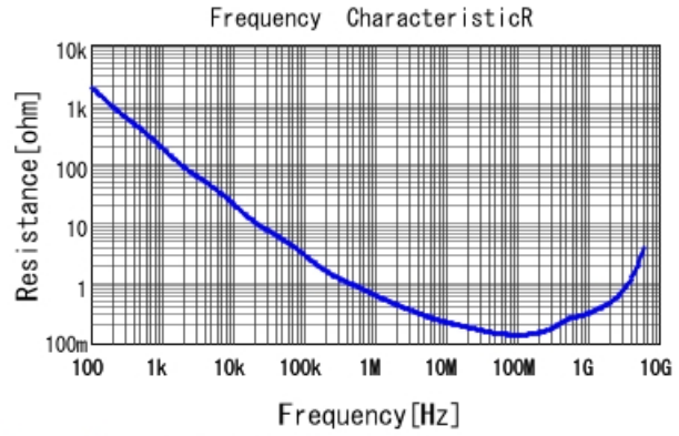
GRM155R71H392KA01 R DCOV, 25degC
