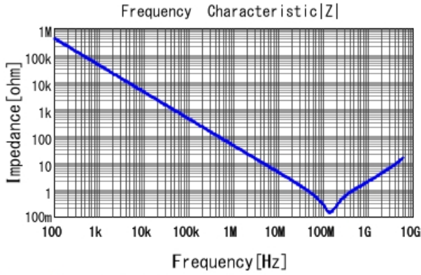
GRM155R71H392KA01 |Z| DCOV, 25degC
