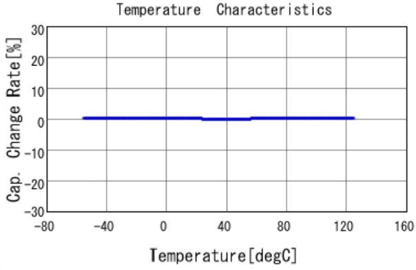
GRM1555C1H1R5WA01 C-Temp. capchange, DCOV, AC1Vrms
