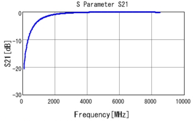
GRM1555C1H1R5WA01 S21 DCOV, 25degC
