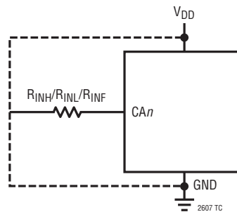
Test Circuit 2
