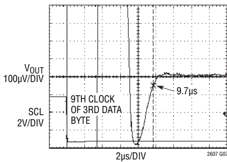
Settling to \pm 1 LSB
