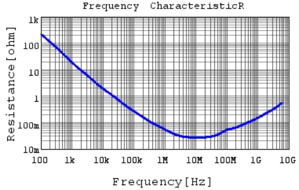
GRM033R60J104KE19 R DCOV, 25degC
