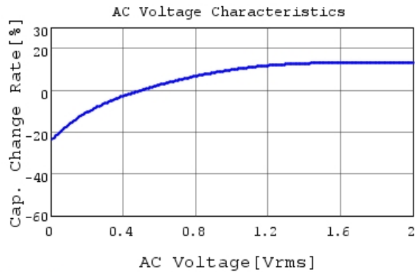
GRM033R60J104KE19 C-AC Voltage capchange, Dc
