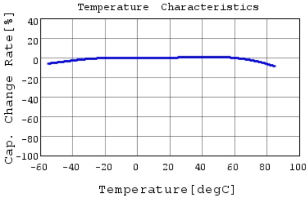
GRM033R60J104KE19 C-Temp. capchange, DC0.0V,
