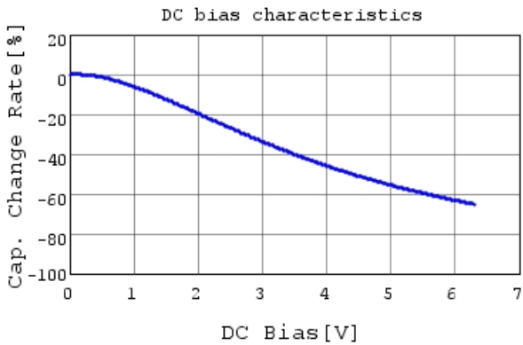
GRM033R60J104KE19 C-DC bias capchange, 25.0c
