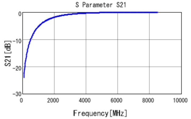
GRM1885C1H1R0WA01 S21 DCOV, 25degC
