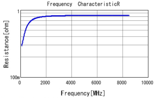
GRM1885C1H1R0WA01 R DCOV, 25degC
