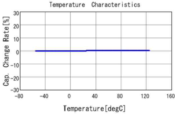
GRM1885C1H1R0WA01 C-Temp. capchange, DCOV, AC1Vrms
