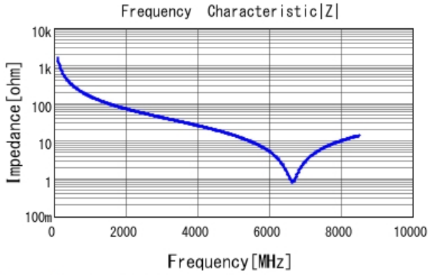
GRM1885C1H1R0WA01 |Z| DCOV, 25degC
