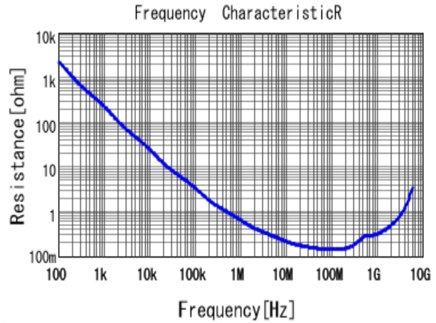
■ GRM155R71H332KA01 R DCOV, 25degC
