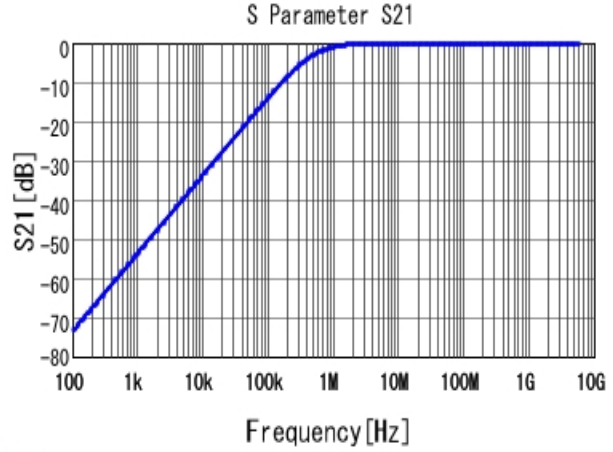
■ GRM155R71H332KA01 S21 DCOV, 25degC
