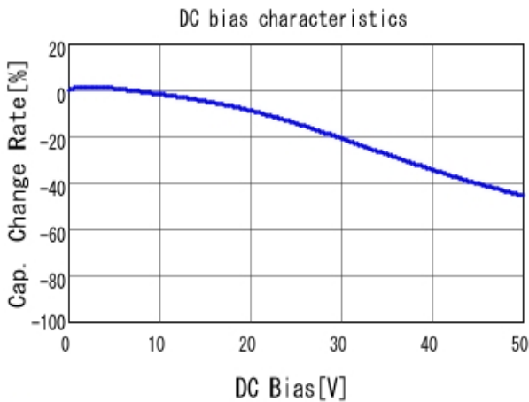
■ GRM155R71H332KA01 C-DC bias capchange, 25.0degC, AC1.
