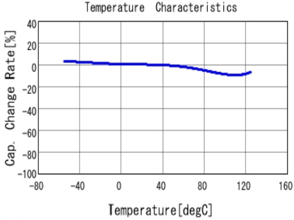
■ GRM155R71H332KA01 C-Temp. capchange, DCO. 0V, AC1.0V rm
