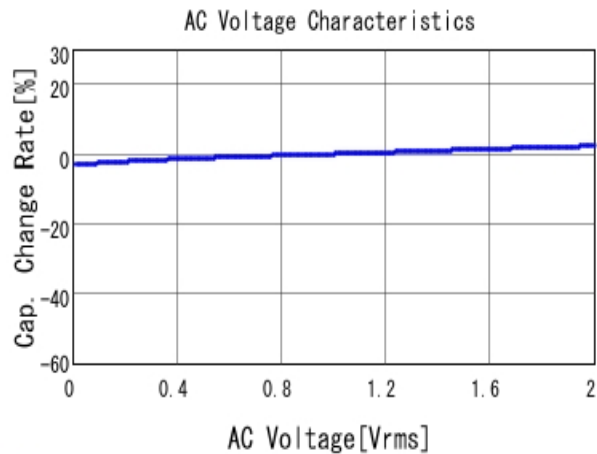
■ GRM155R71H332KA01 C-AC Voltage capchange, DCOV, 25.0d
