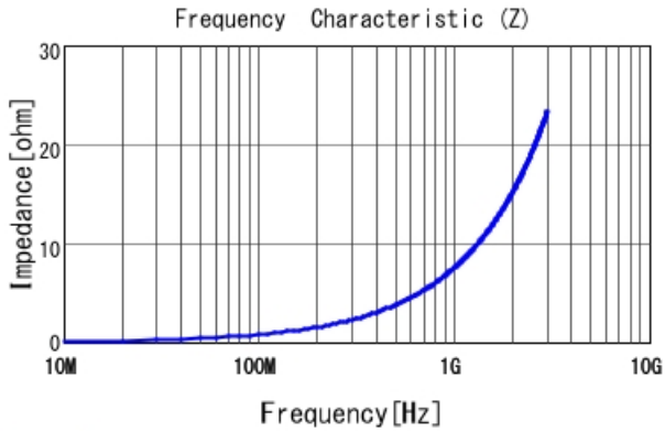
LQP03HQ1N2W02 |Z|
