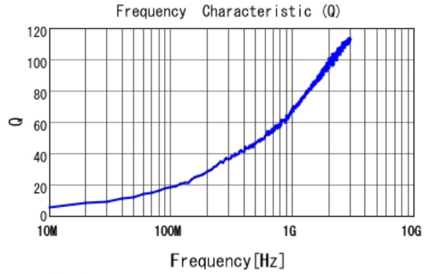
LQP03HQ1N2W02 Q
