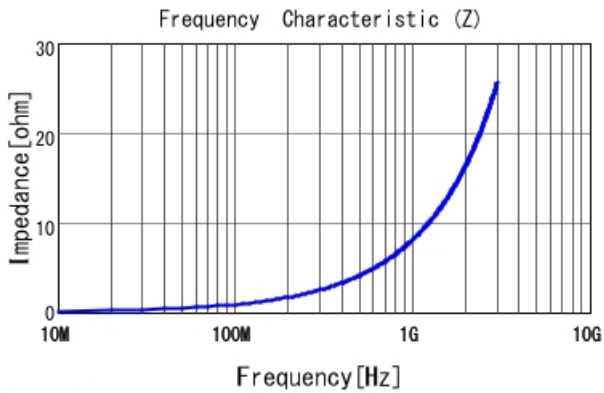
LQP03TG1N3C02 |Z|
