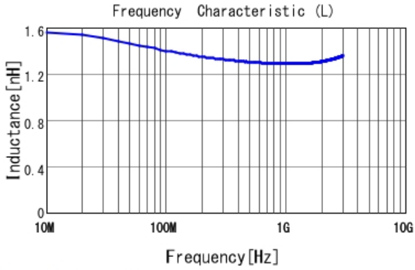
LQP03TG1N3C02 L
