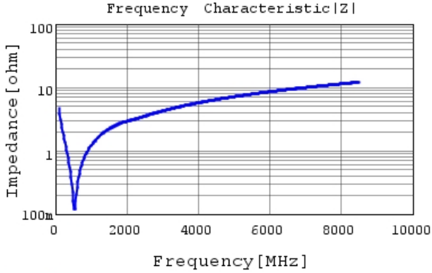
GRM0335C1E331GA01 |Z| DCOV, 25degC
