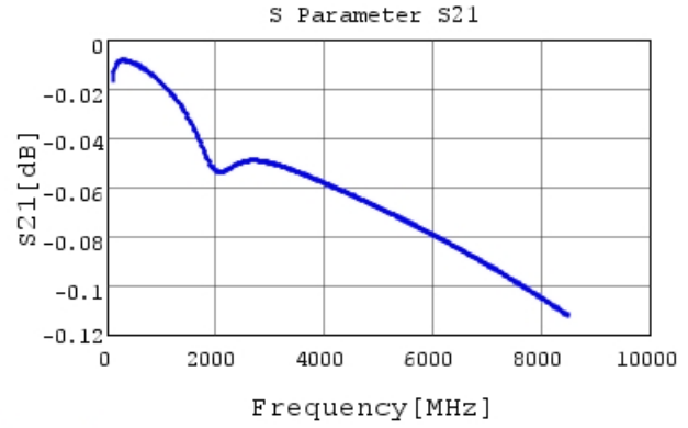
GRM0335C1E331GA01 S21 DCOV, 25degC
