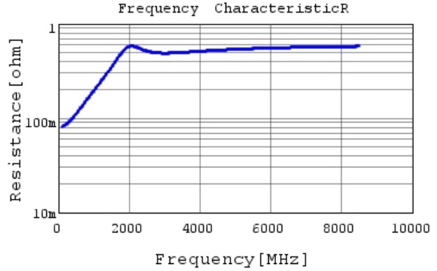
GRM0335C1E331GA01 R DCOV, 25degC
