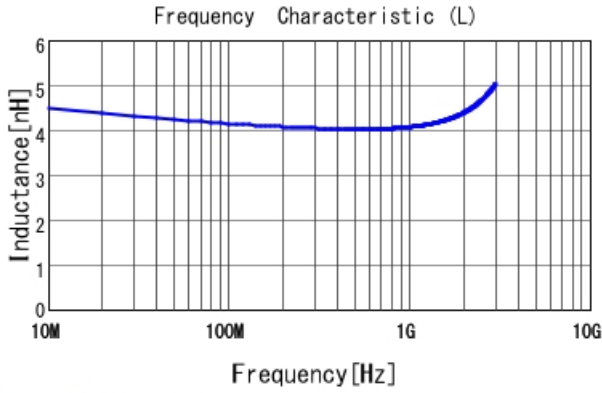
LQG15WZ4N1B02 L
