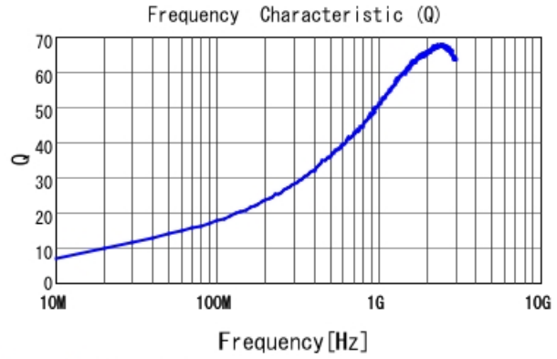
LQG15WZ4N1B02 Q
