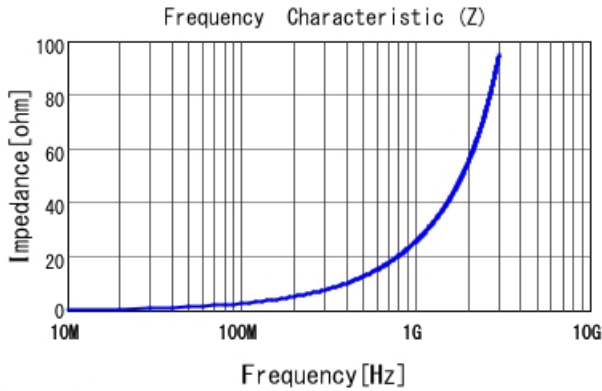
LQG15WZ4N1B02 |Z|
