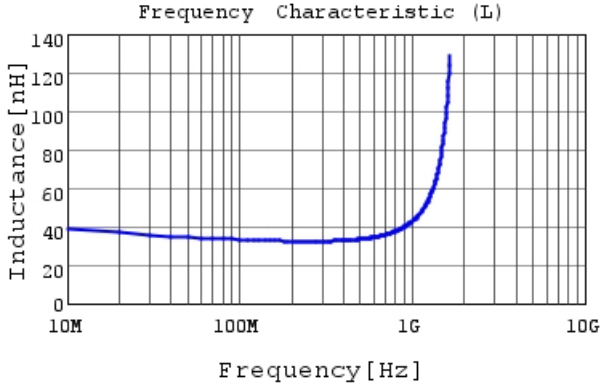
LQG15HN33NJ02 L
