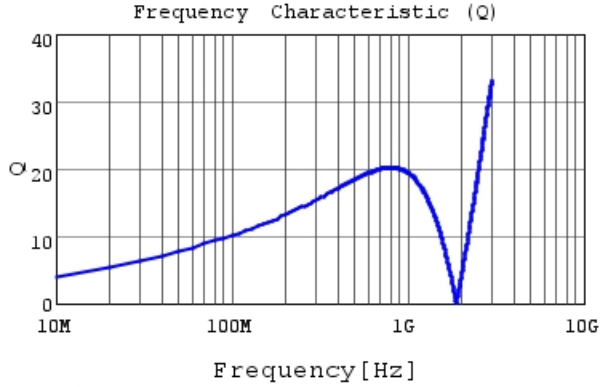
LQG15HN33NJ02 Q
