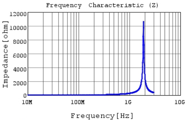
LQG15HN33NJ02 |Z|
