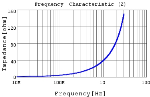
LQP03TG6N2J02 |Z|
