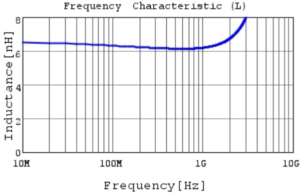
LQP03TG6N2J02 L
