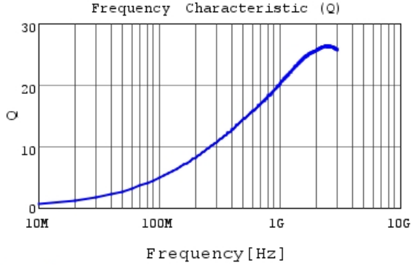
LQP03TG6N2J02 Q
