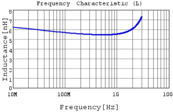
LQG15HN5N6C02 L
