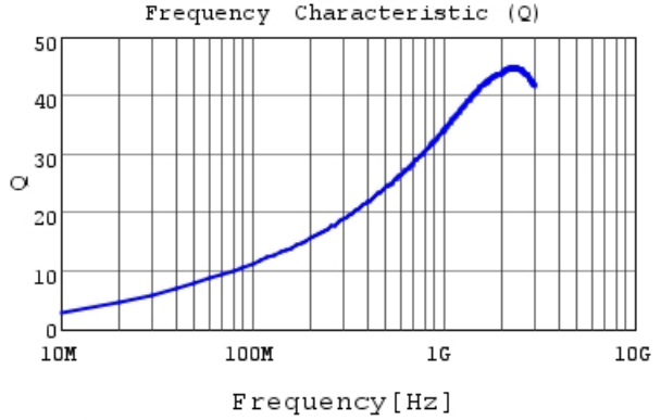
LQG15HN5N6C02 Q
