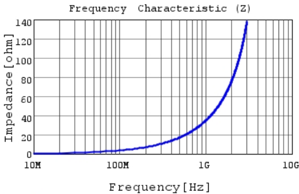
LQG15HN5N6C02 |Z|
