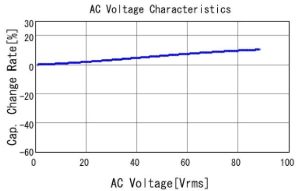
GCJ21AR72E102KXJ1 C-AC Voltage capchange, DCOV, 25
