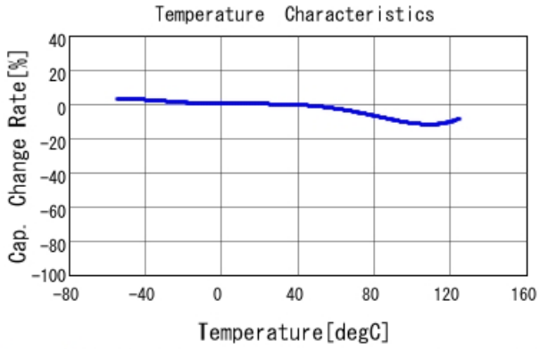
GCJ21AR72E102KXJ1 C-Temp. capchange, DCOV, AC1Vrms
