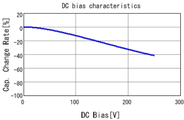
GCJ21AR72E102KXJ1 C-DC bias capchange, 25.0degC, A
