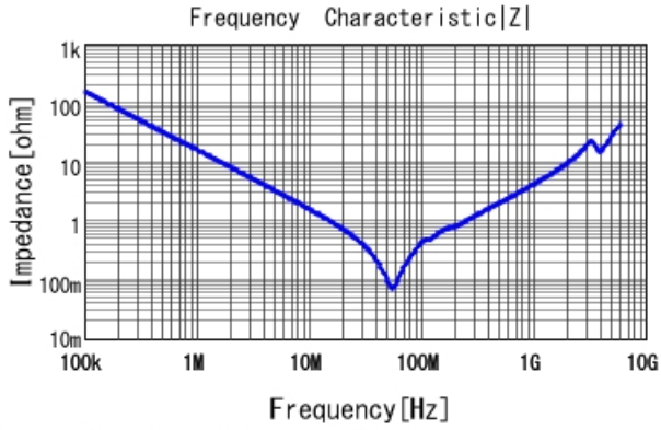
GRM31CR73A103KW03 |Z| DCOV, 25degC
