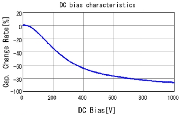
GRM31CR73A103KW03 C-DC bias capchange, 25.0degC, A
