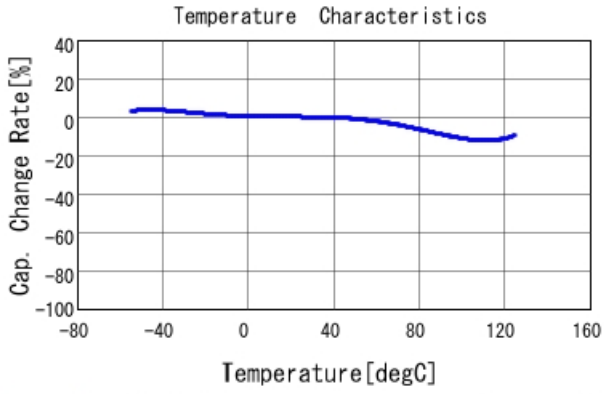
GRM31CR73A103KW03 C-Temp. capchange, DCOV, AC1Vrms
