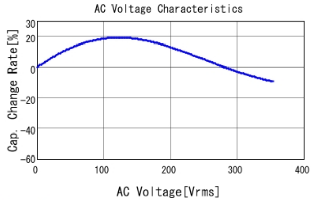
GRM31CR73A103KW03 C-AC Voltage capchange, DCOV, 25
