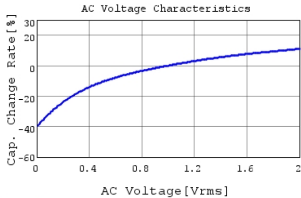
GRT155R61E224KE01 C-AC Voltage capchange, Dc
