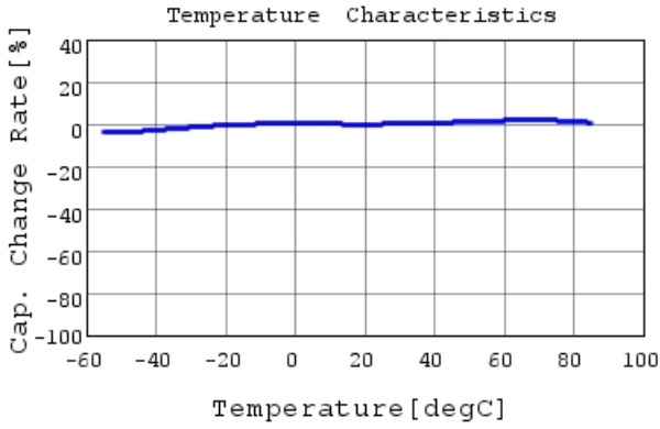
GRT155R61E224KE01 C-Temp. capchange, DC0.0V,
