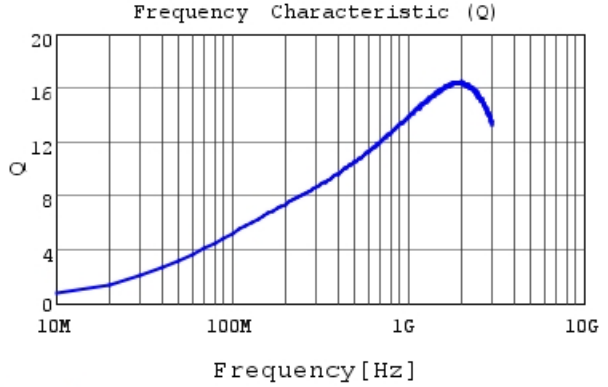
LQP02TQ20NJ02 Q
