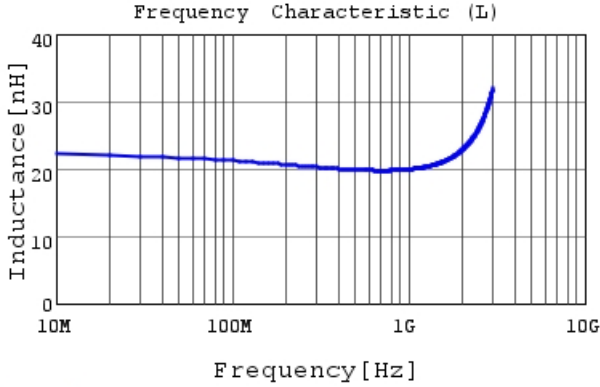
LQP02TQ20NJ02 L
