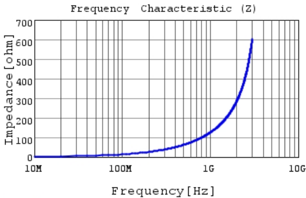
LQP02TQ20NJ02 |Z|
