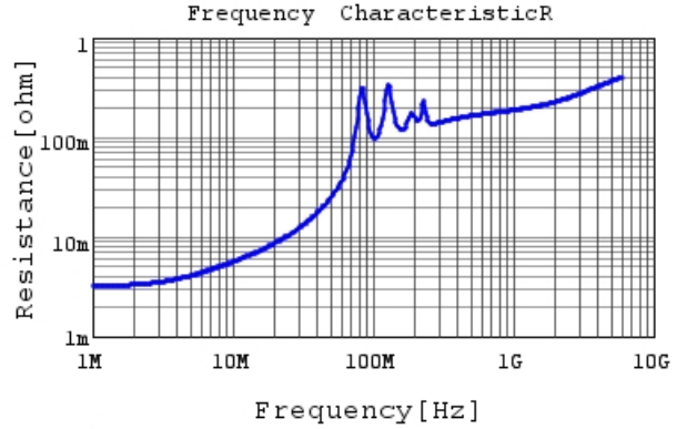
GRM21B2C1H223JA01 R DCOV, 20degC
