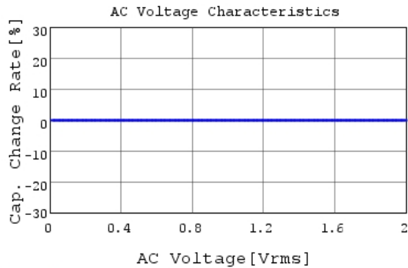
GRM21B2C1H223JA01 C-AC Voltage capchange, Dc
