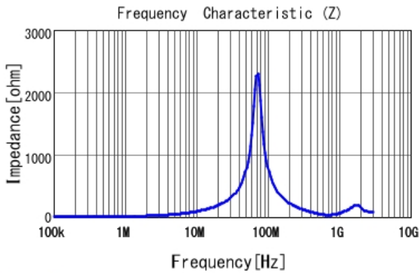
1267AY-1R5N |Z|
