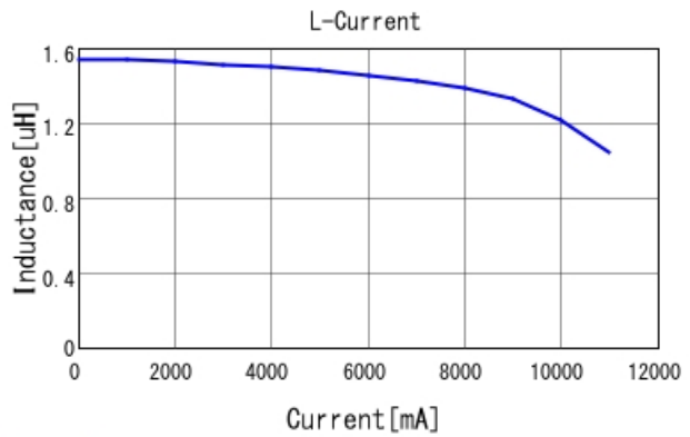
1267AY-1R5N L-Current 20degC
