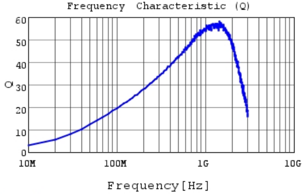
LQW15AN62NJ00 Q
